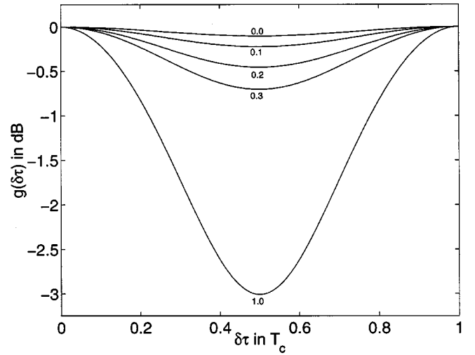
Fig. 9. Energy of chip-sampled raised cosine g(\delta\tau) versus chip mismatch \delta\tau for different rolloff factors.
